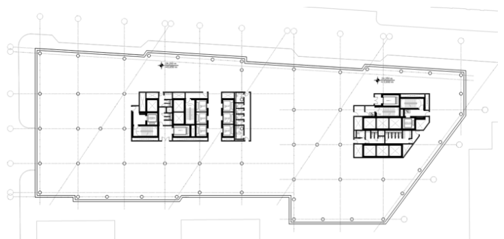
Figure 4: Mapping of the tower grid onto the podium grid, © Ramboll
